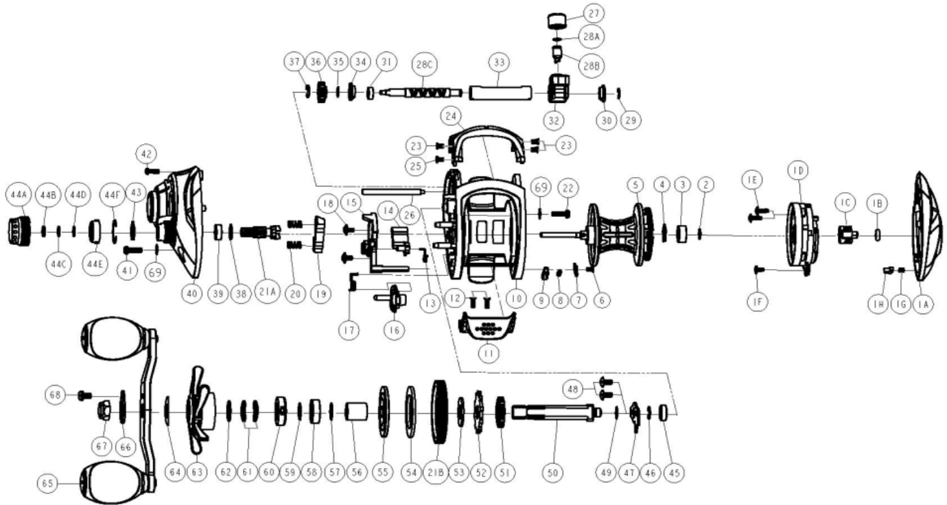
Quantum Energy T101HPTMg Baitcast Reel Part List
