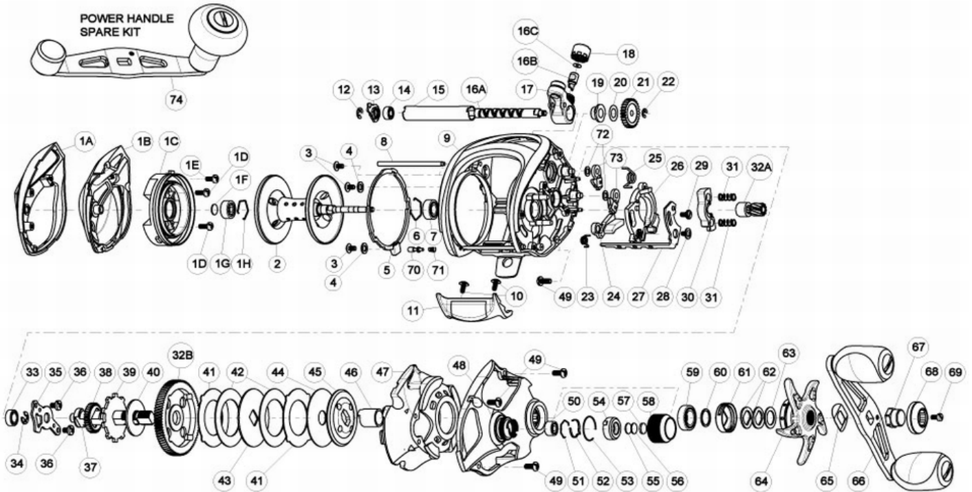
Quantum EX300SPT Bait Cast Reel Part List
