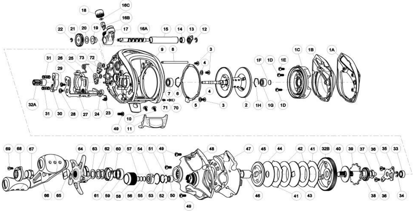
Quantum EX201HPT Bait Cast Reel Part List
