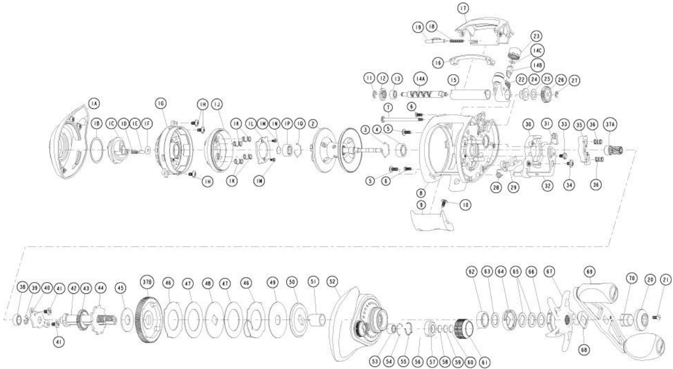
Quantum SL150SPT Bait Cast Reel Part List
